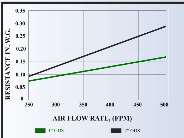
STANDARD PRESSURE DROP Test Filter Size 24" x 24" Nominal
