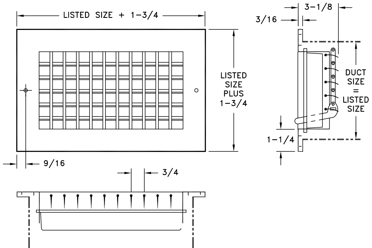
VM VERTICAL FACE BARS
