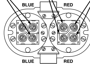
No. 5 Switch Used on 93, 193, 94 and 194 Series.
