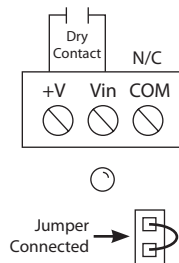
Example of Dry Contact Input Operation
