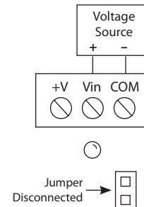
Example of Voltage Input Operation
