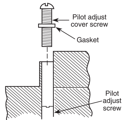
Figure 5. Pilot gas adjustment
