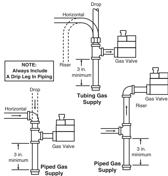
Figure 1. Typical gas valve piping
