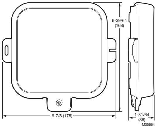
Fig. 15. Dimensions.
